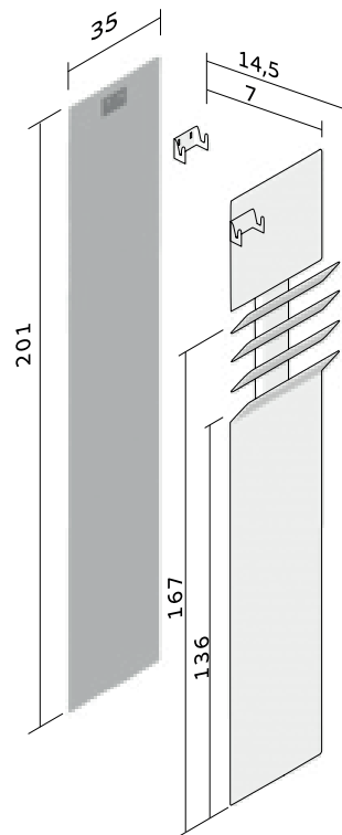
Flaps A
