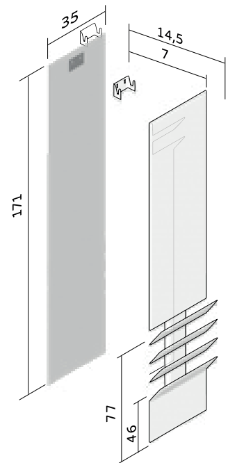
Flaps B
